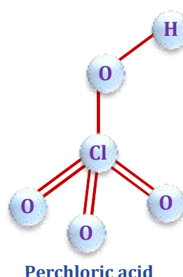
The structures of oxyacids of chlorine
