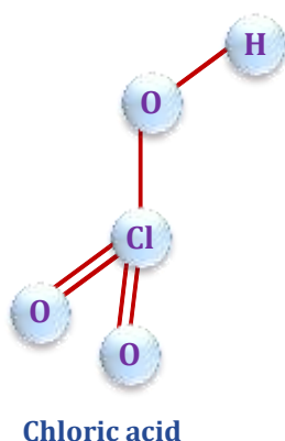
The structures of oxyacids of chlorine
