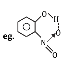
o-nitrophenol
