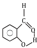
Salicylaldehyde
