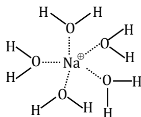
Hydration of Na^+
