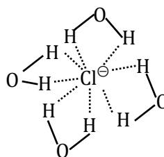
Hydration of Cl^-
