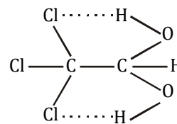
Chloral hydrate
